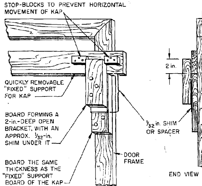
Fig. B-19. Quick-removal bracket.
